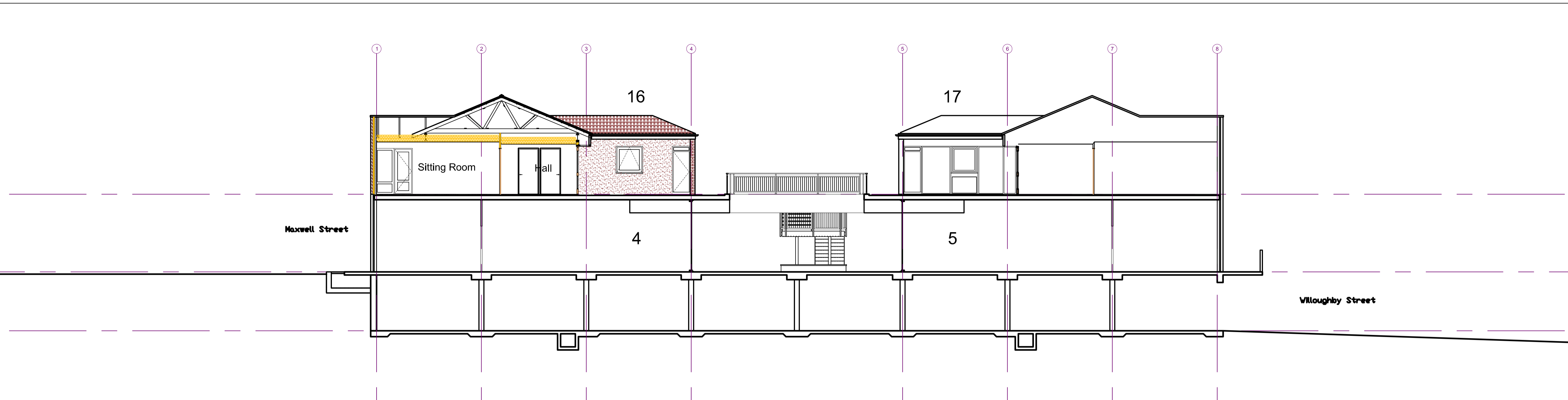
North Section BB
