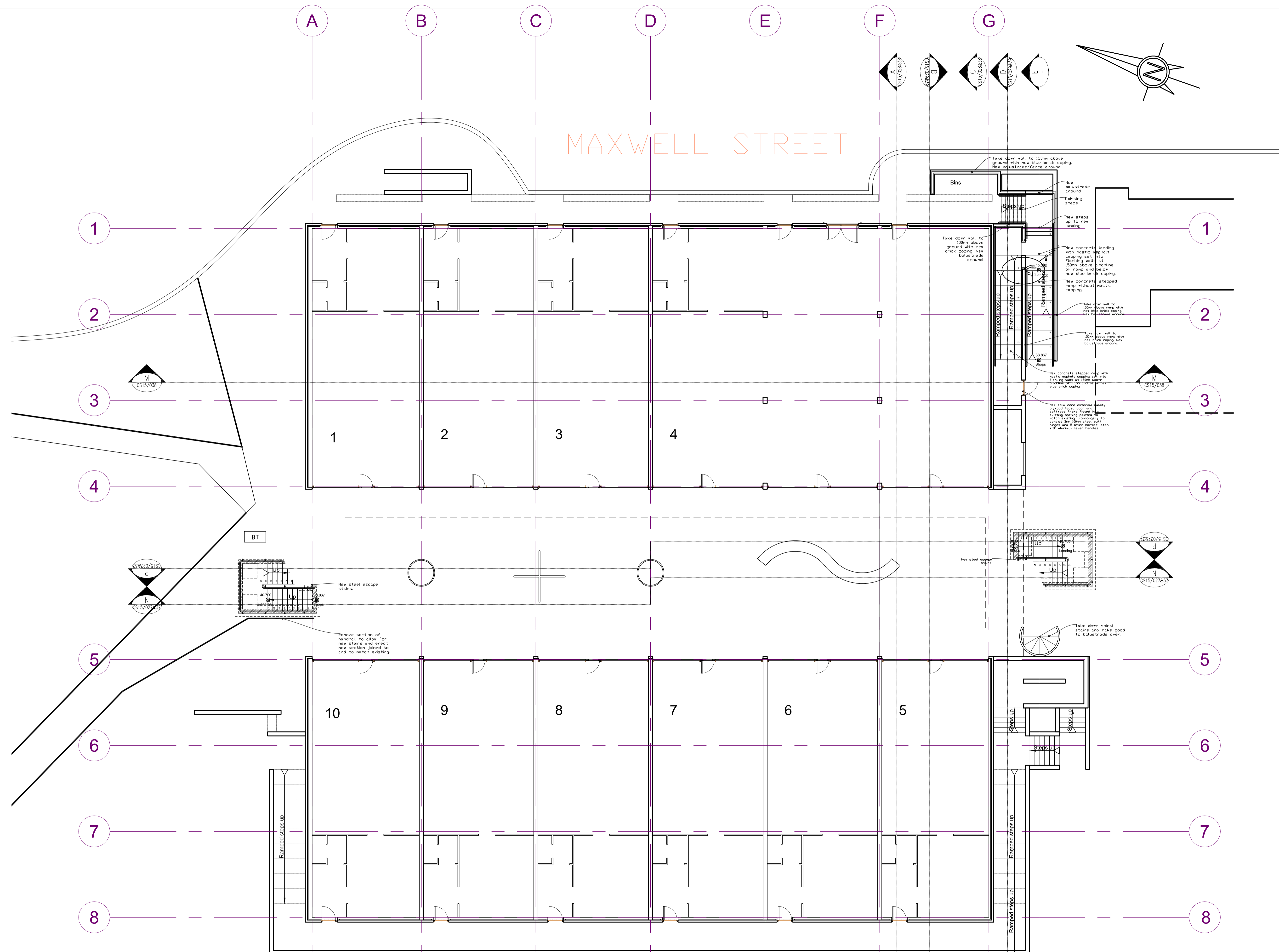
Ground floor plan - Shops
